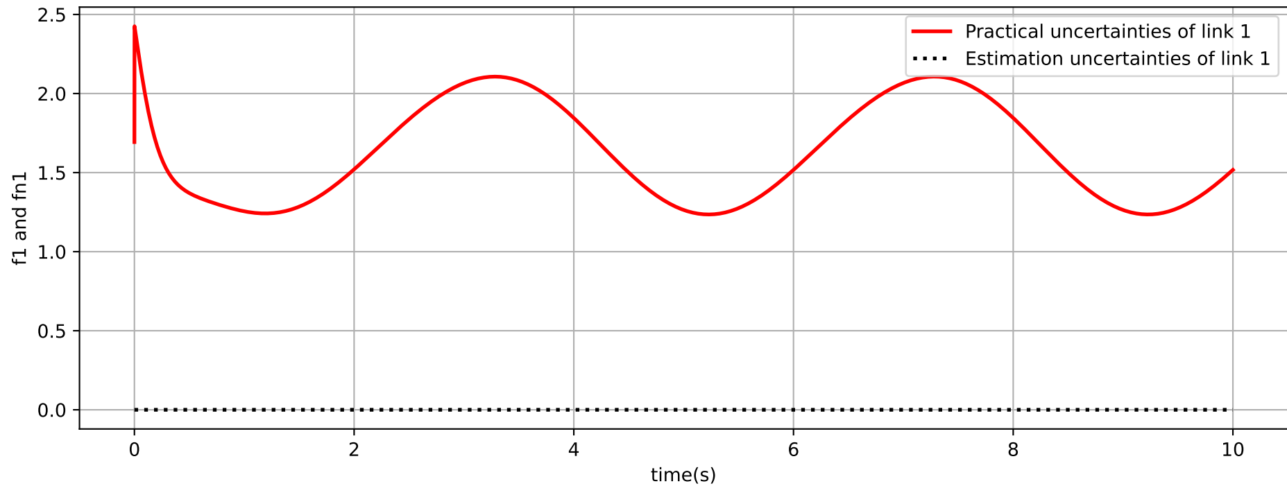
Disturbance Estimation Performance (S=2, S1=1, m=5)
